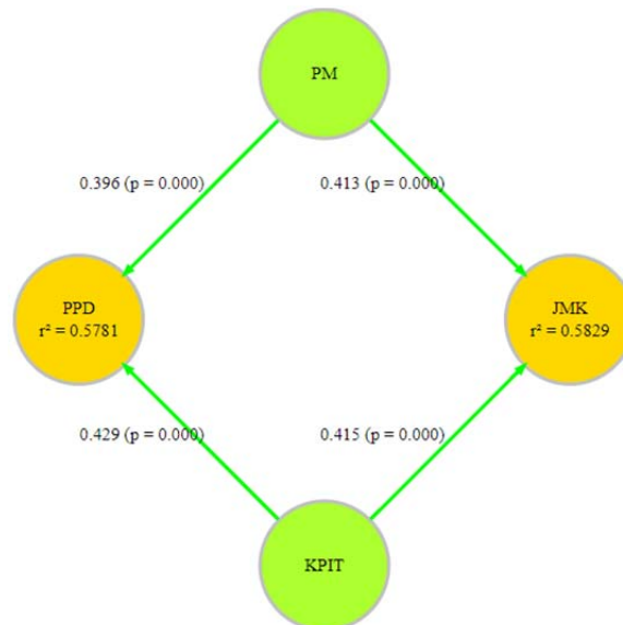
Figure 3. Significance Testing
